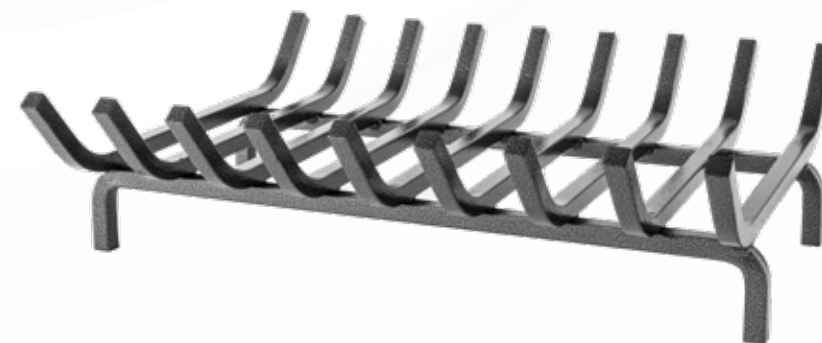
BR651 BRACIERE 9 BARRE - QUADRO 14 / 9 STICKS LOG GRATE - ROUND 14 Dimensioni / Dimensions: L: 50 P: 40 H: 14 cm Peso / Weight: 8 kg
